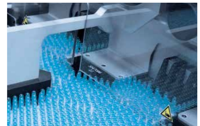
Ampoule Infeed Standing Ampoules are delivered via a feeding table to the pick and place handling units
